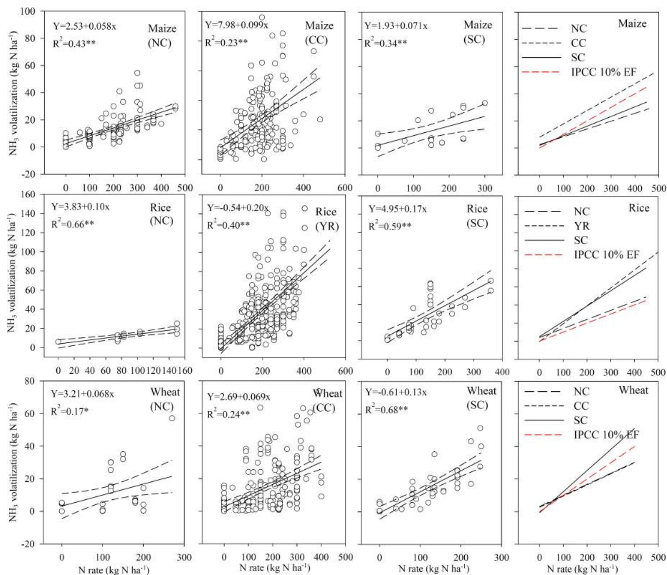
Extended Data Figure 5 | Linear models describing the relationship between \text{NH}_3 volatilization and nitrogen rate. \text{NH}_3 -N volatilization was plotted against nitrogen rate for maize ( n = 315 ), rice ( n = 423 ) and wheat ( n = 279 ) growing seasons, respectively. The red dotted line is the IPCC
